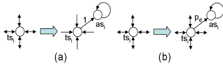
Figure 6. (a) If ts_i is covered by any sensor, then a new absorbing state as_i is added. The transition probability from ts_i to as_i is 1 if the penetrator at ts_i can be always detected. (b) If ts_i is covered by two sensors. Assume each sensor is being active with probability p . We have a new state transition diagram shown in the right with p_d(ts_i) = 1 - (1 - p)^2 .
