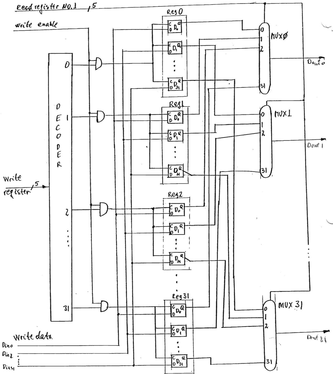
MIPS Register file with 32 32-bit registers Design at the level of flip-flop, decoder & multiplexers
