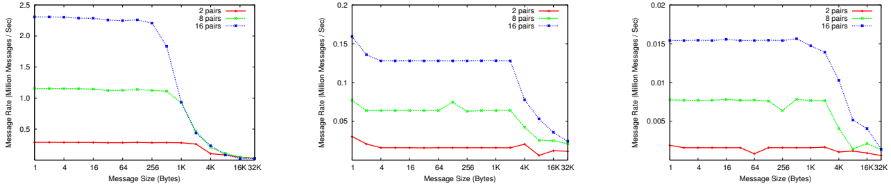
Figure 6. Multi-pair message rate for varying delays: (a) 100us delay (b) 1ms delay (c) 10ms delay
