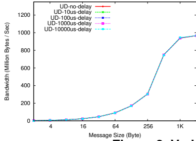
Figure 2. Verbs level throughput using (a) UD (b) RC
