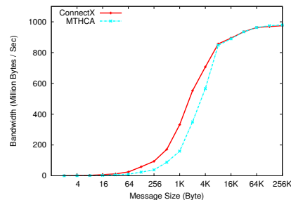
Figure 10. Verbs level RC Bandwidth
