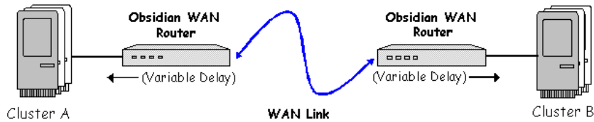
Figure 1. Cluster-of-Clusters Connected with Obsidian Longbow XR Routers
