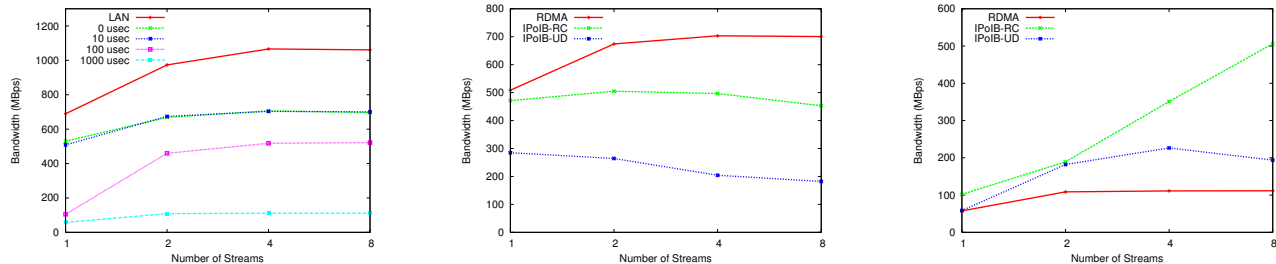
Figure 9. NFS Read throughput of (a) NFS over RDMA, (b) NFS over RDMA and IPoIB with 10 us delay and (c) NFS over RDMA and IPoIB with 1000 us delay
