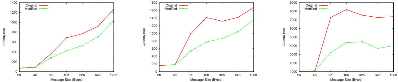
Figure 7. MPI broadcast latency over IB WAN: (a) 10us delay (b) 100us delay (c) 1000us delay
