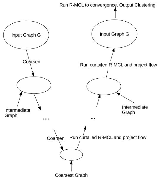
Figure 1: A high-level overview of Multi-level Regularized MCL.
