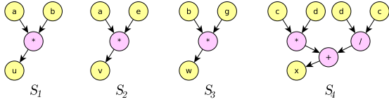
Fig. 3: Evaluating S_4 before S_{1,2,3} reduces register pressure
