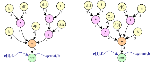
(a) Tree with context at root (b) Optimal schedule
