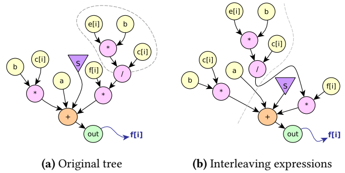
Figure 5. Example: interleaving to reduce MAXLIVE
