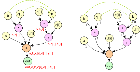
(a) Tree with data sharing (b) Scheduling cost
