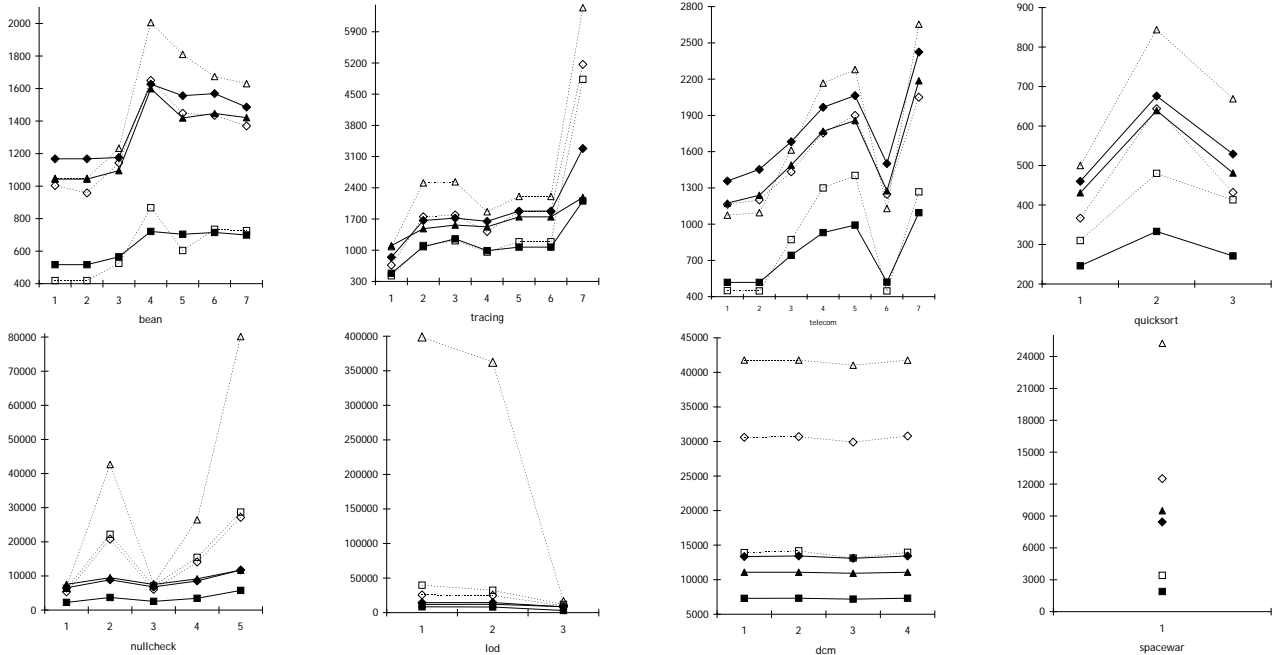
Figure 6. ICFG edges □/■, control-dependence ◇/◆ and data-dependence △/▲ edges: woven bytecode (□, ...) and AJANA (■, ...)
