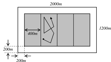
Figure 15. The simulation scenario for scalability. The event is limited to move only within a small gray rectangle in each simulation.
