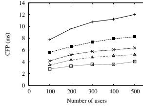
Fig. 8. Multicast AP=75.
