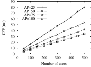
Fig. 9. Unicast.
