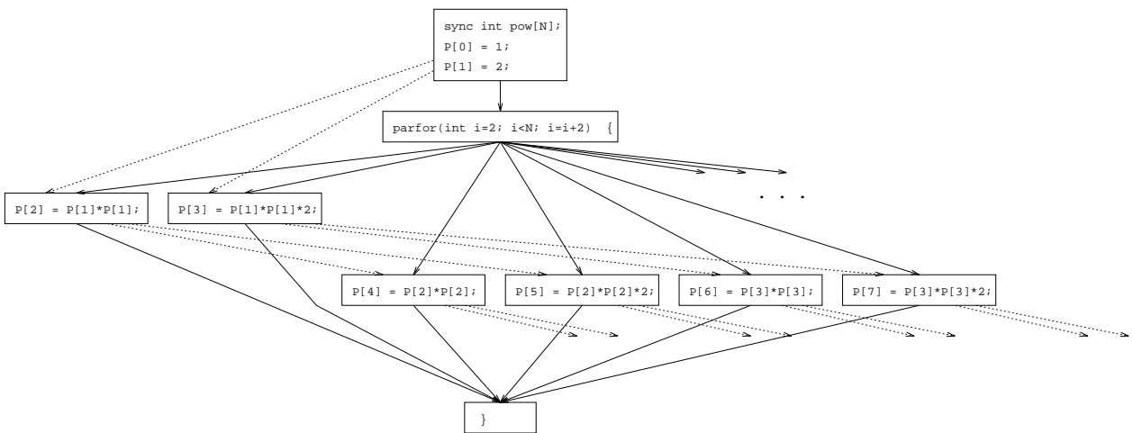
Figure 4.3: Binary Tree Data Dependency for Calculating Powers of 2
