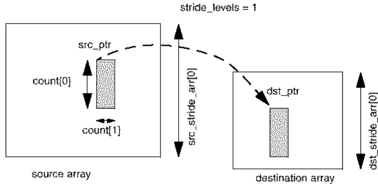
Fig. 2. Strided format for 2-dimensional array sections (assuming Fortran layout).
