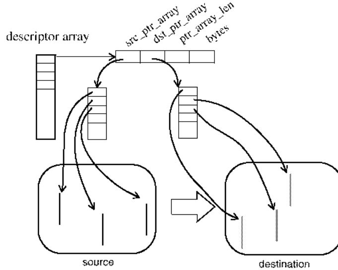
Fig. 1. Descriptor array for generalized I/O vector format. Each array element describes transfer of a set of equally-sized ( bytes ) blocks of data.
