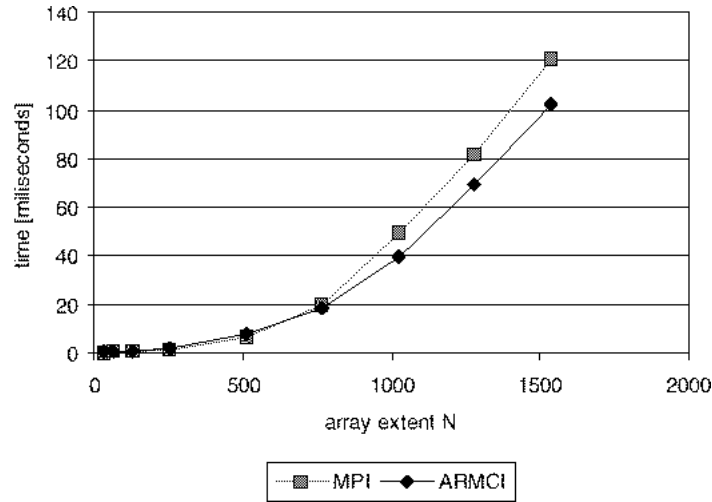
Fig. 6. Timings for original MPI vs new ARMCI implementation of remap . The operation is a particular redistribution of an N by N array.
