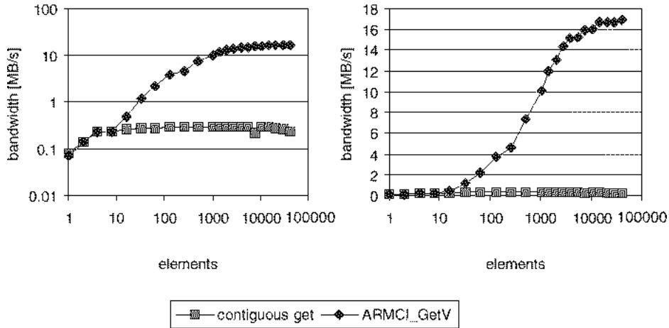
Fig. 5. The log-log (left) and linear-log (right) graphs represent bandwidth in gather operations for double precision numbers as a function of the number of elements when implemented with contiguous get operations and the ARMCI vector get.
