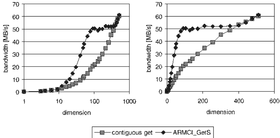
Fig. 4. The log-linear (left) and linear-linear (right) graphs represent bandwidths for a contiguous get operation and ARMCI strided get when moving square sections of a 2-D array.
