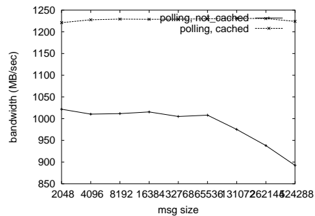
Figure 11. Emulating RDMA Write over UD (a) Latency (b) Bandwidth
