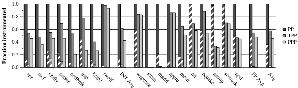
Figure 11. The fraction of dynamic paths instrumented by PP, TPP, and PPP. The stripes represent hashed paths.
