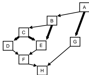
Figure 4. Example routine with all obvious paths. Each path has at least one defining edge (marked in bold).
