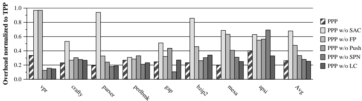
Figure 13. PPP leave-one-out methodology normalized to TPP. SAC = Self-adjusting cold edge criterion; FP = Free cold path poisoning; Push = Pushing instrumentation further; SPN = Smart path numbering; LC = Instrument routines with low coverage only.
