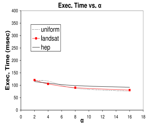
Figure 12: Execution Time as a function of \alpha .
