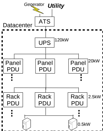
Power delivery system in our CSE department's DC
