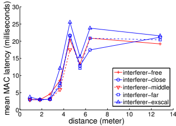
Figure 14: MAC latency in the presence of interference
