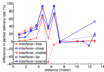
Figure 6: The difference between broadcast and unicast in different interfering scenarios
