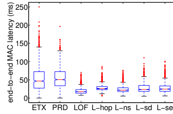
Figure 17: End-to-end MAC latency
