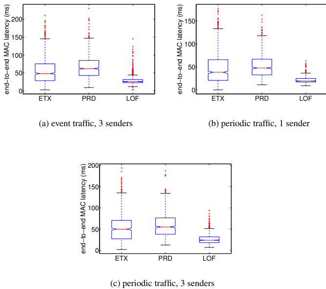
Figure 24: End-to-end MAC latency
