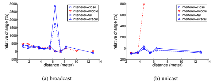
Figure 8: Relative change in the COV of packet delivery rate
