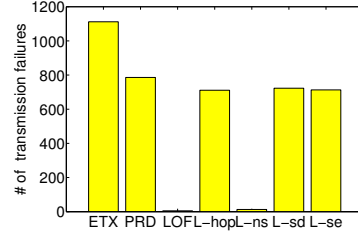
Figure 23: Number of failed unicast transmissions
