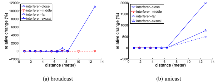
Figure 7: Relative change in packet delivery rate
