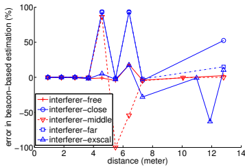
Figure 9: Error in estimating unicast delivery rate via that of broadcast
