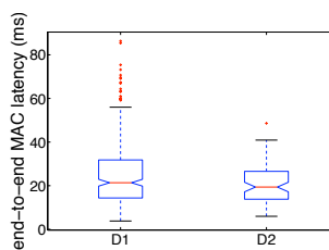
Fig. 8. End-to-end MAC latency
