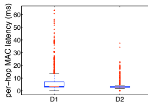
Fig. 7. Per-hop MAC latency
